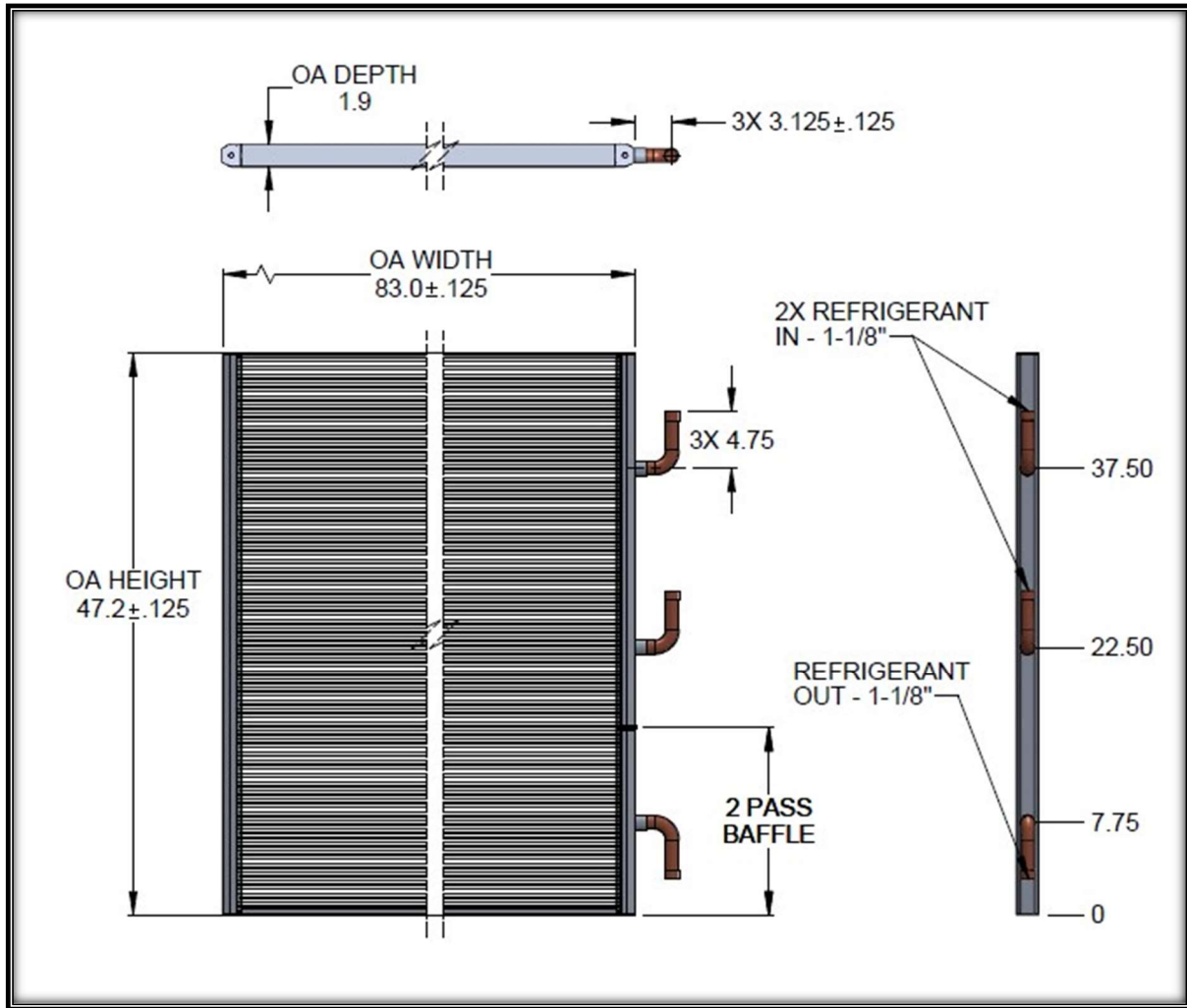
Figure 1. Model: C46.4x80.8x1.25H-24E07-V4297C (Epoxy Coated)
