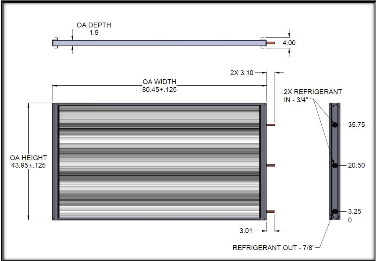
Figure 1. Model: C42.8x76x1.25H-24B05-J3514C (Epoxy Coated)
