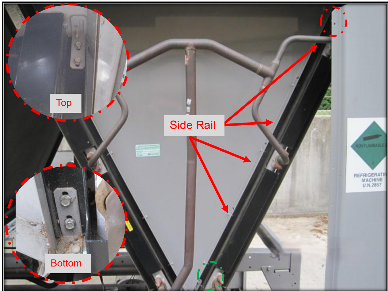
Figure 3. Screw Locations: Top – 1, Bottom – 3, Side rail – 5
