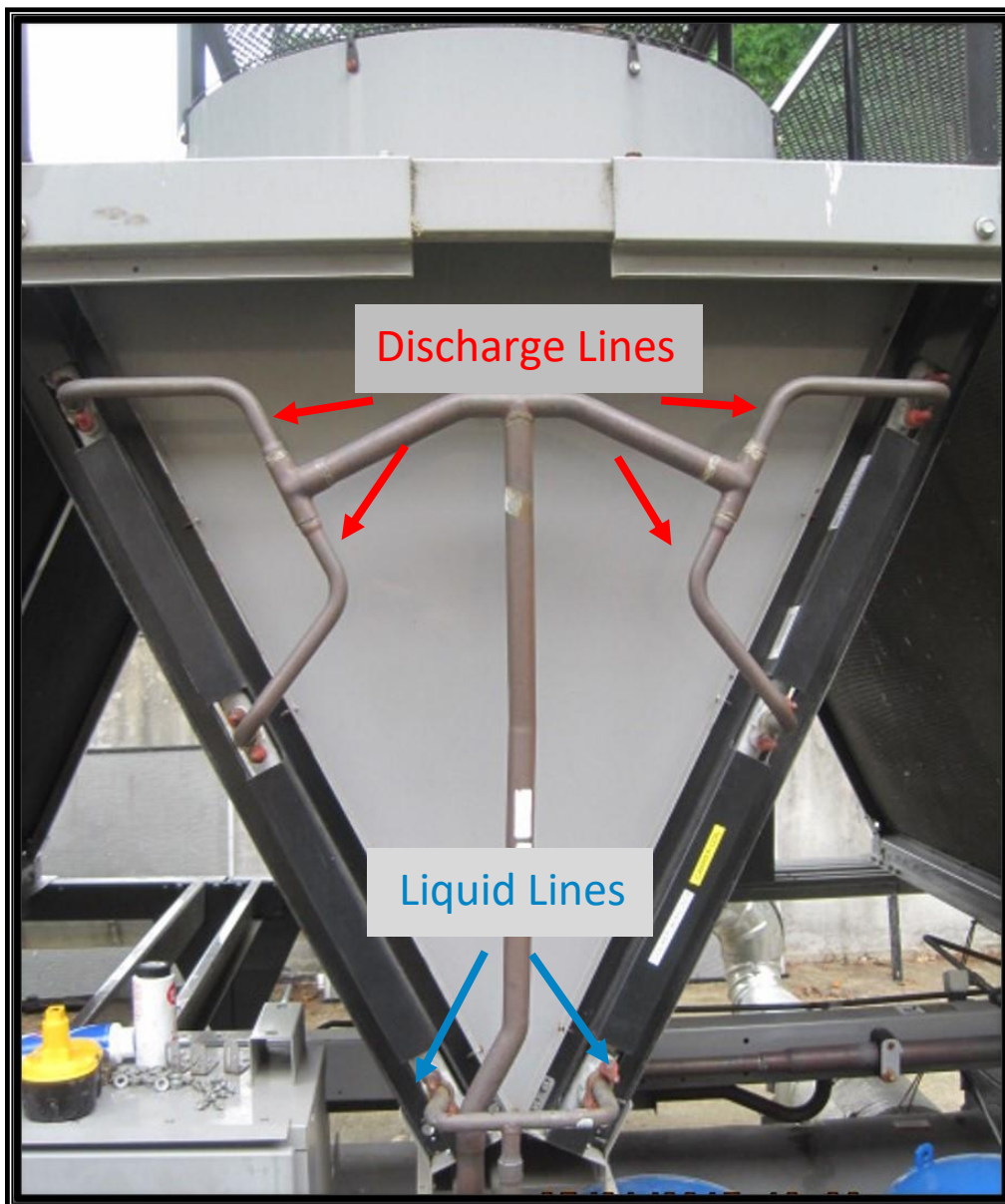
Figure 2. Front of Chiller
