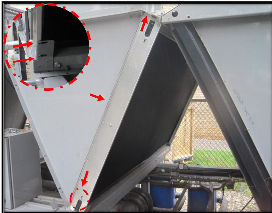
Figure 7. Back of Chiller: Secure the Coil Through the Flanges.
